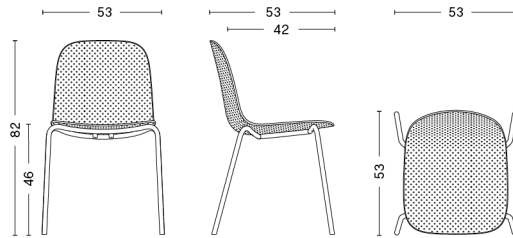
STEEL FRAME CHAIR
