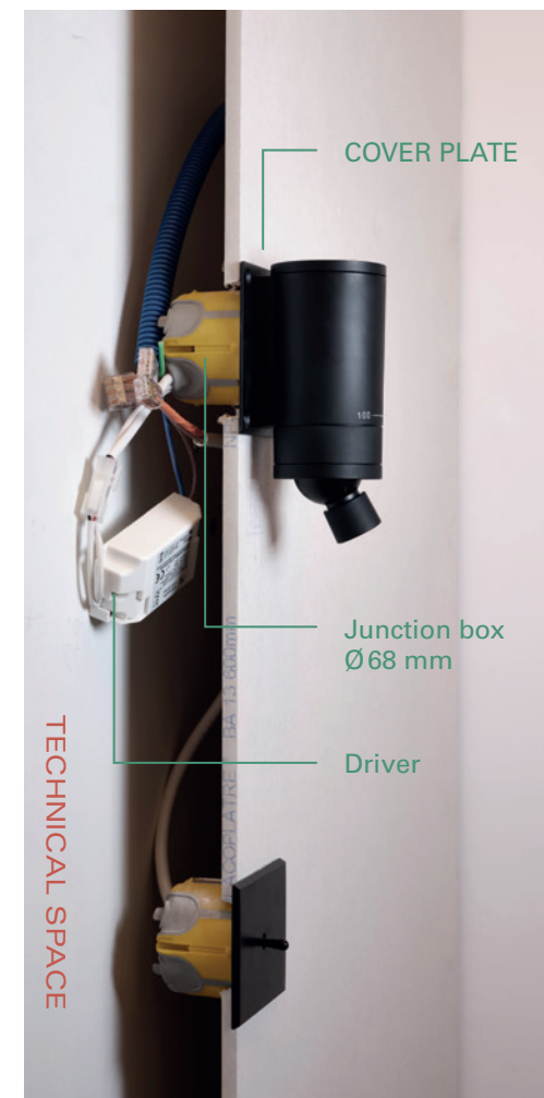
VISION 20/20 OMNI with junction box Ø68 mm, use the COVER PLATE
