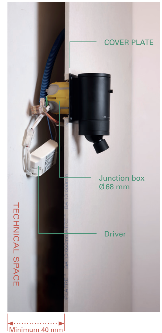
VISION 20/20 OMNI SW with junction box Ø 68 mm, use the COVER PLATE
