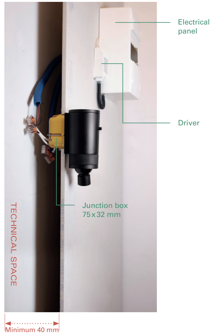
VISION 20/20 OMNI SW with separated driver
