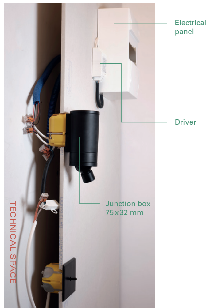
VISION 20/20 OMNI with separated driver
