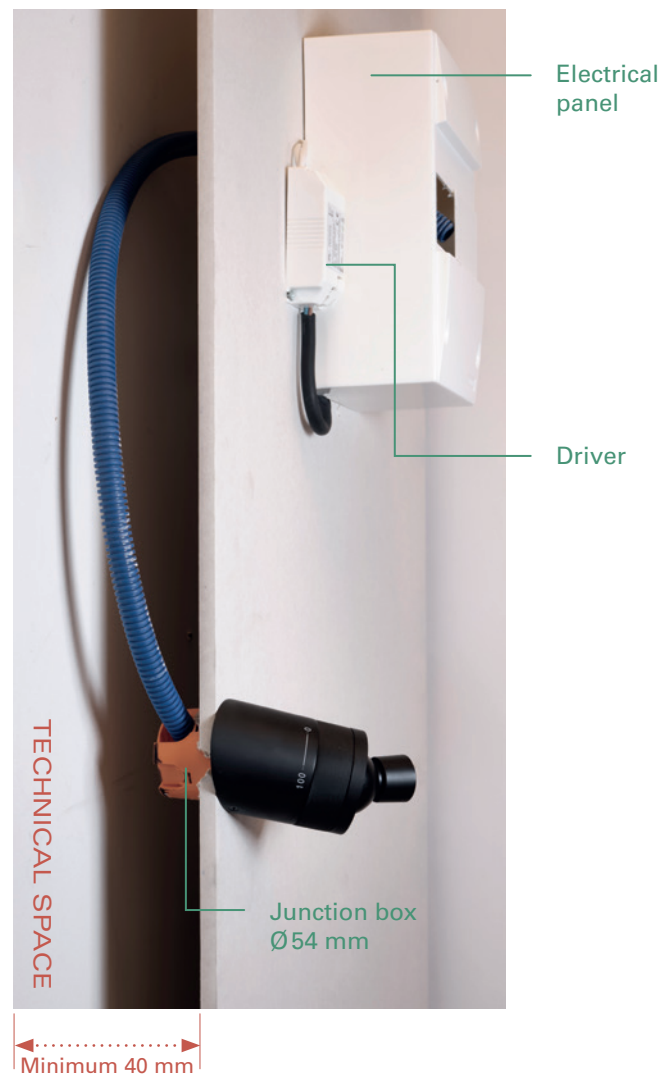
VISION 20/20 SW with separated driver
